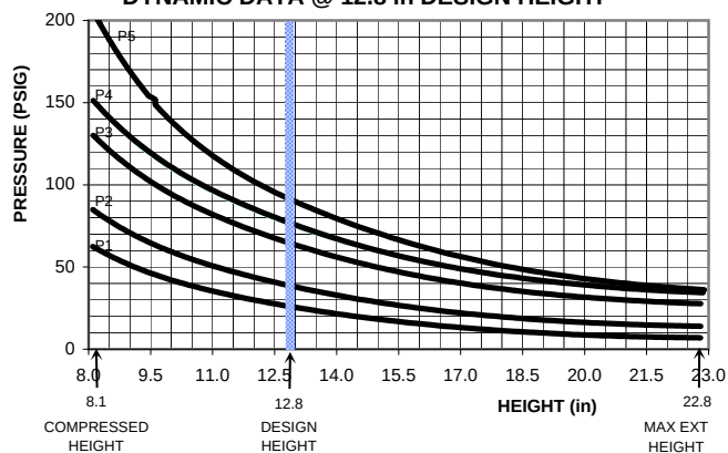
DYNAMIC DATA @ 12.8 in DESIGN HEIGHT
