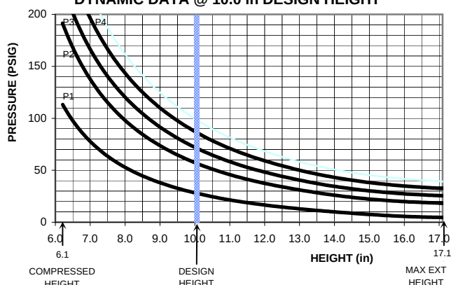
DYNAMIC DATA @ 10.0 in DESIGN HEIGHT
