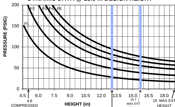
DYNAMIC DATA @ 13.0 in DESIGN HEIGHT
