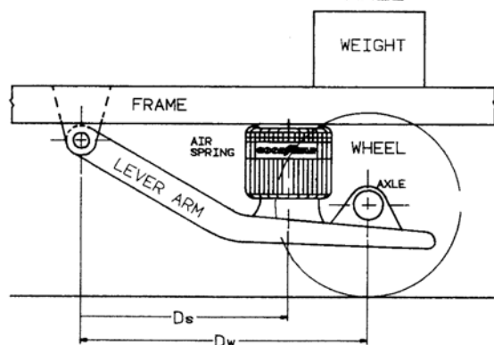
SPRING AHEAD OF AXLE
