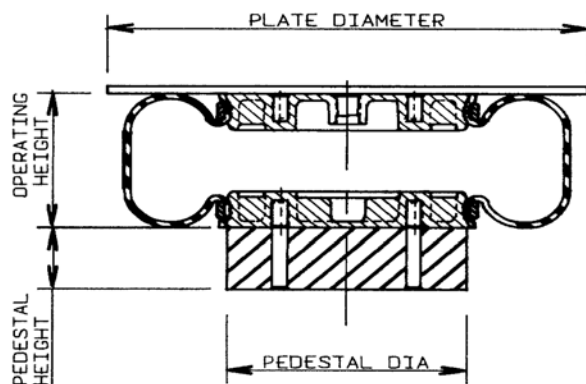
PEDESTAL REQUIRED WHEN OPERATING SPRING AT OR BELOW HEIGHTS LISTED IN THE TABLE
