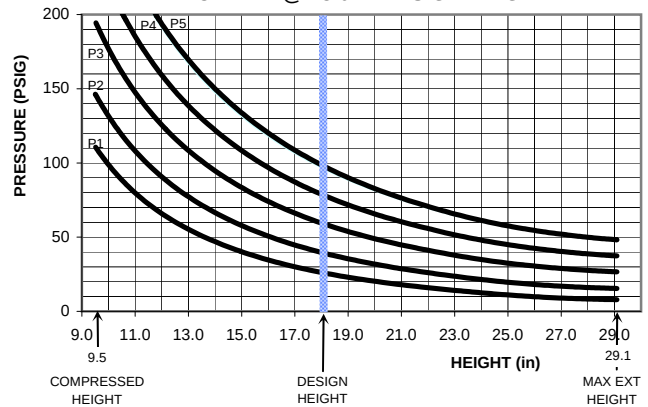
DYNAMIC DATA @ 18.0 in DESIGN HEIGHT
