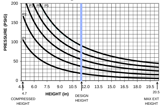
DYNAMIC DATA @ 11.5 in DESIGN HEIGHT
