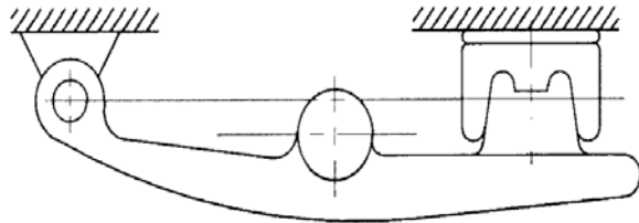
Fig. 5.1 Rolling Lobe fully compressed
