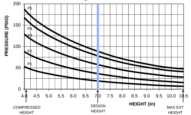
DYNAMIC DATA @ 7.0 in DESIGN HEIGHT
