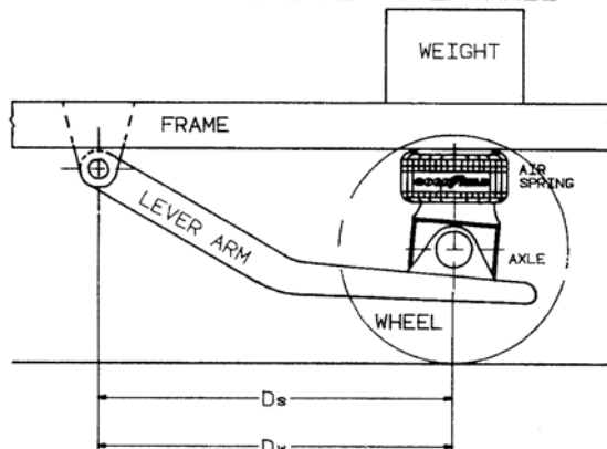
SPRING DIRECTLY OVER AXLE
