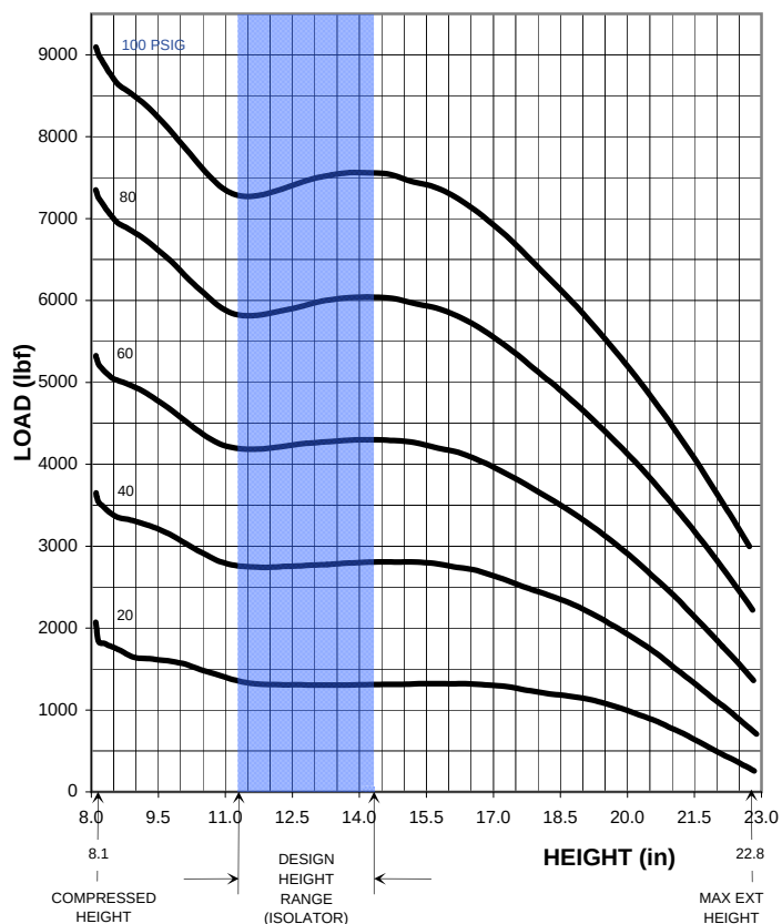
LOAD vs. DEFLECTION @ CONSTANT PRESSURE
