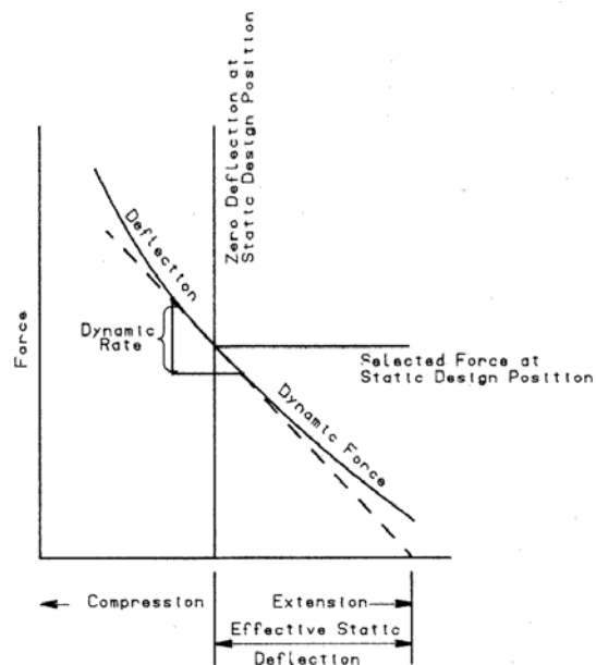
Fig. 2.1 Effective static deflection
