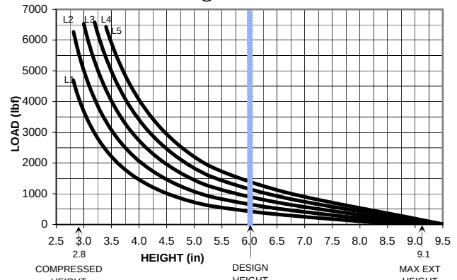
DYNAMIC DATA @ 6.0 in DESIGN HEIGHT
