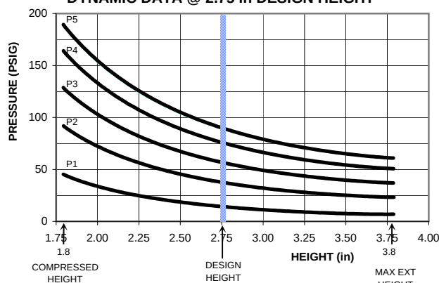
DYNAMIC DATA @ 2.75 in DESIGN HEIGHT
