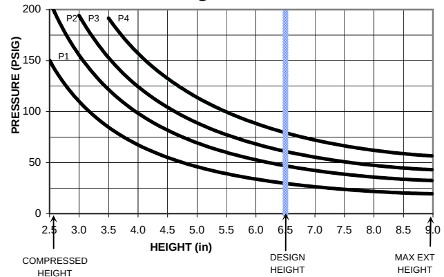
DYNAMIC DATA @ 6.5 in DESIGN HEIGHT
