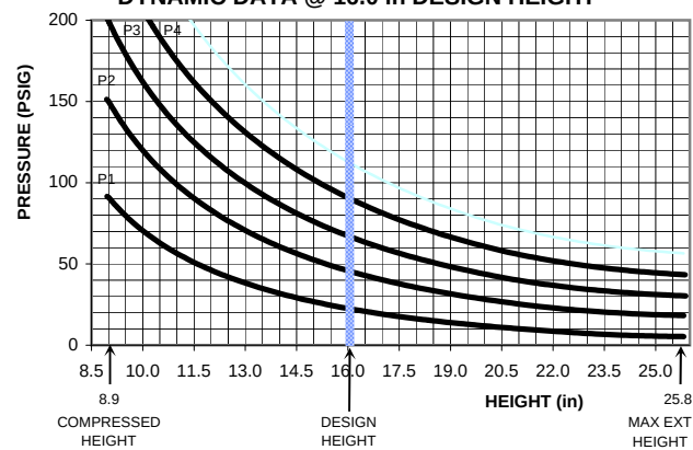
DYNAMIC DATA @ 16.0 in DESIGN HEIGHT
