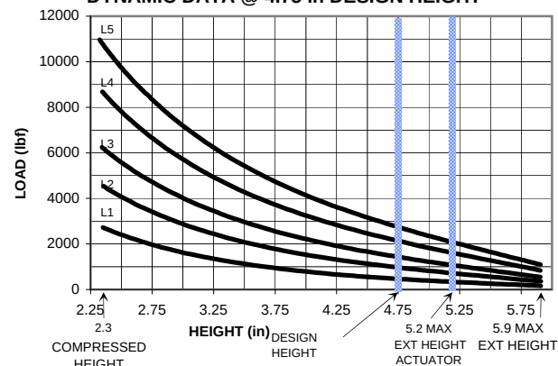
DYNAMIC DATA @ 4.75 in DESIGN HEIGHT
