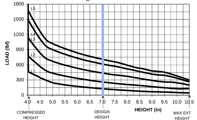
DYNAMIC DATA @ 7.0 in DESIGN HEIGHT
