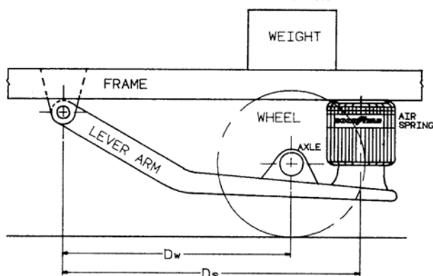
SPRING BEHIND AXLE
