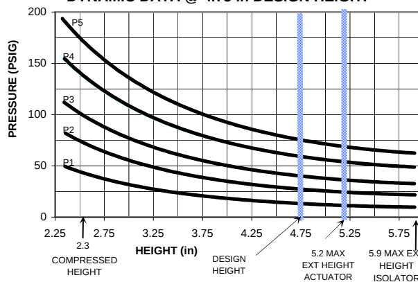
DYNAMIC DATA @ 4.75 in DESIGN HEIGHT
