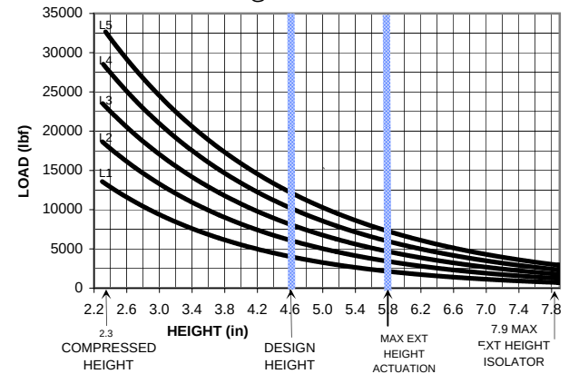
DYNAMIC DATA @ 4.6 in DESIGN HEIGHT
