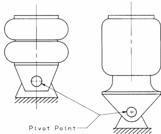
Fig. 5.9 Unstable mounting
