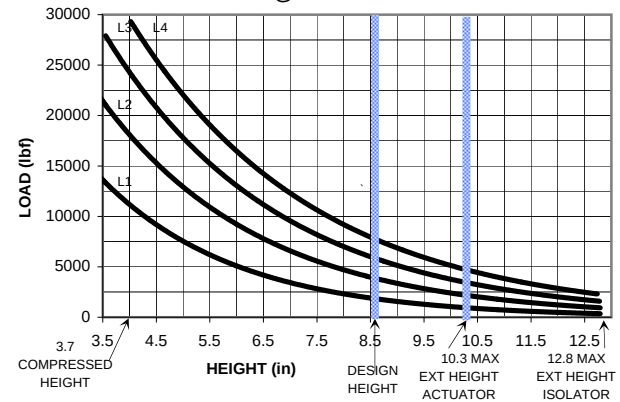
DYNAMIC DATA @ 8.5 in DESIGN HEIGHT
