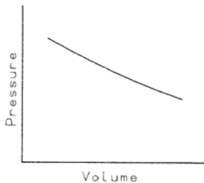
Fig. 2.4 Constant temperature non-flow process (isothermal process)
