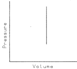
Fig. 2.3 Constant volume, non-flow process
