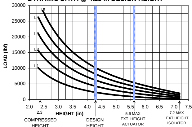
DYNAMIC DATA @ 4.25 in DESIGN HEIGHT
