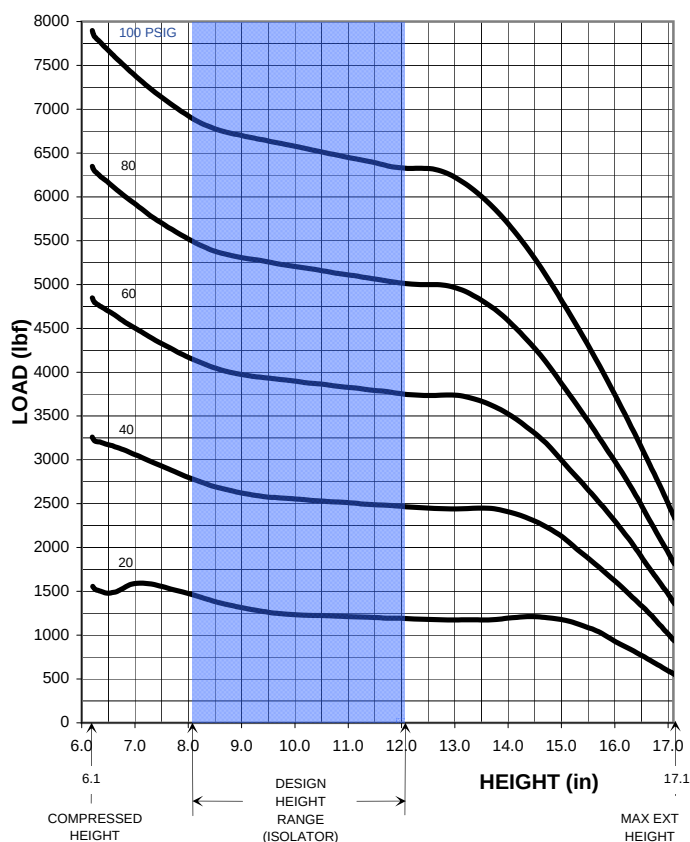
LOAD vs. DEFLECTION @ CONSTANT PRESSURE
