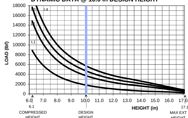
DYNAMIC DATA @ 10.0 in DESIGN HEIGHT
