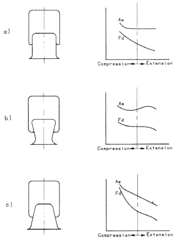
Fig. 2.2 Characteristic variations due to piston shapes and flexible member size
